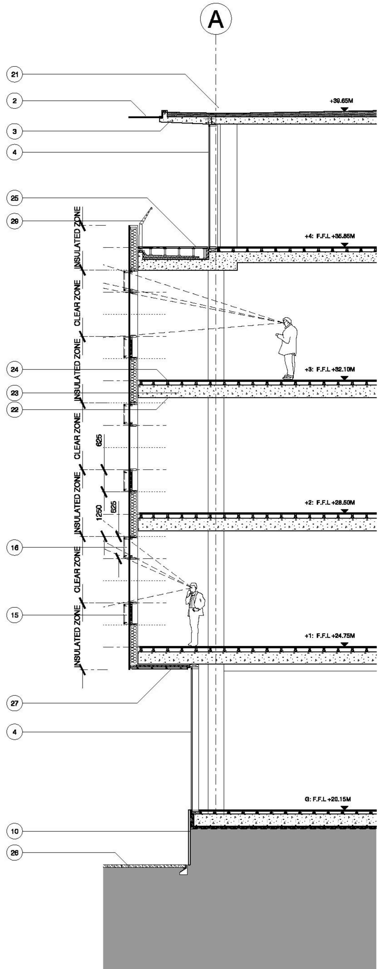
02 DETAIL SECTION
