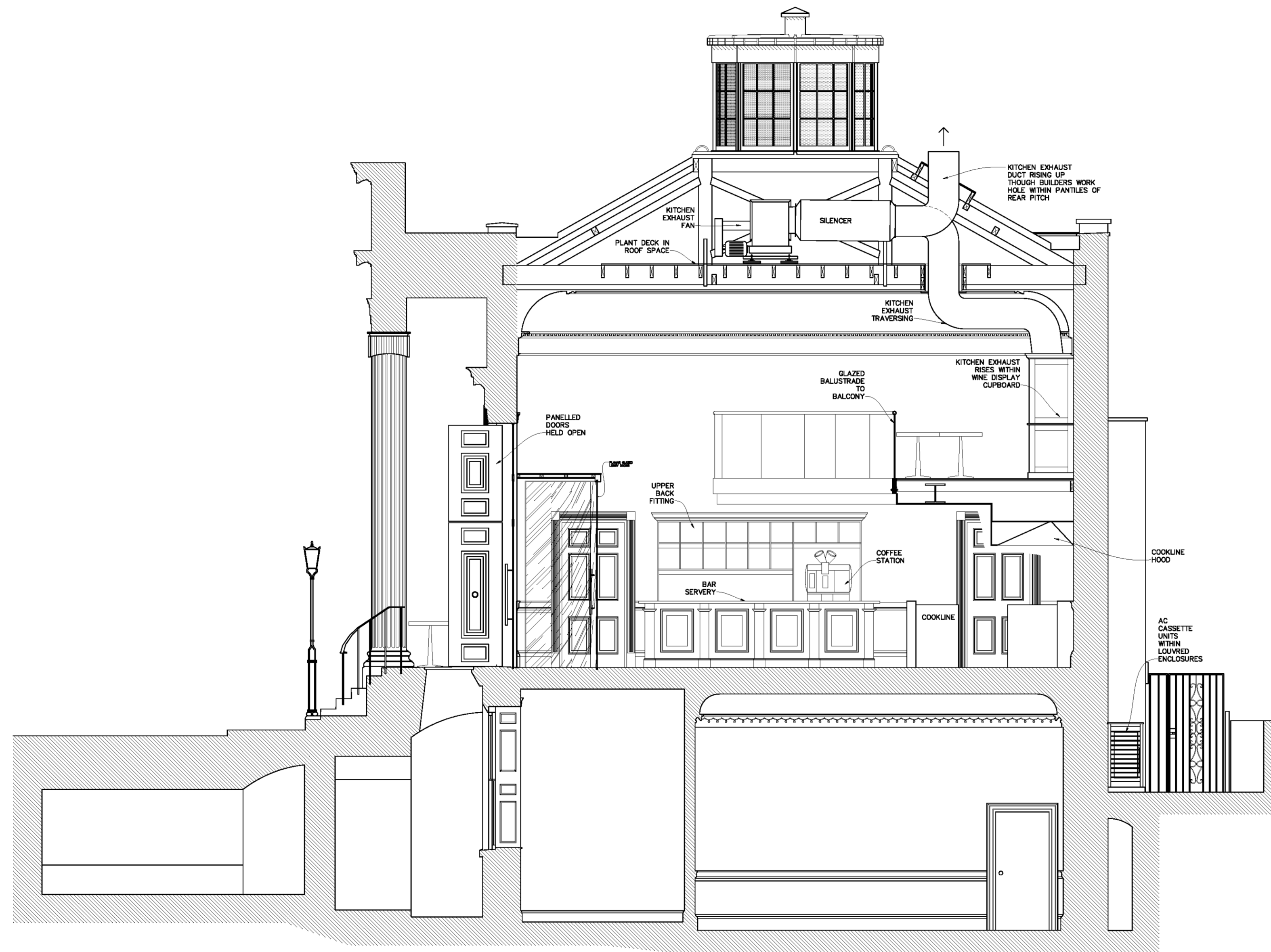
PROPOSED SECTION EE
