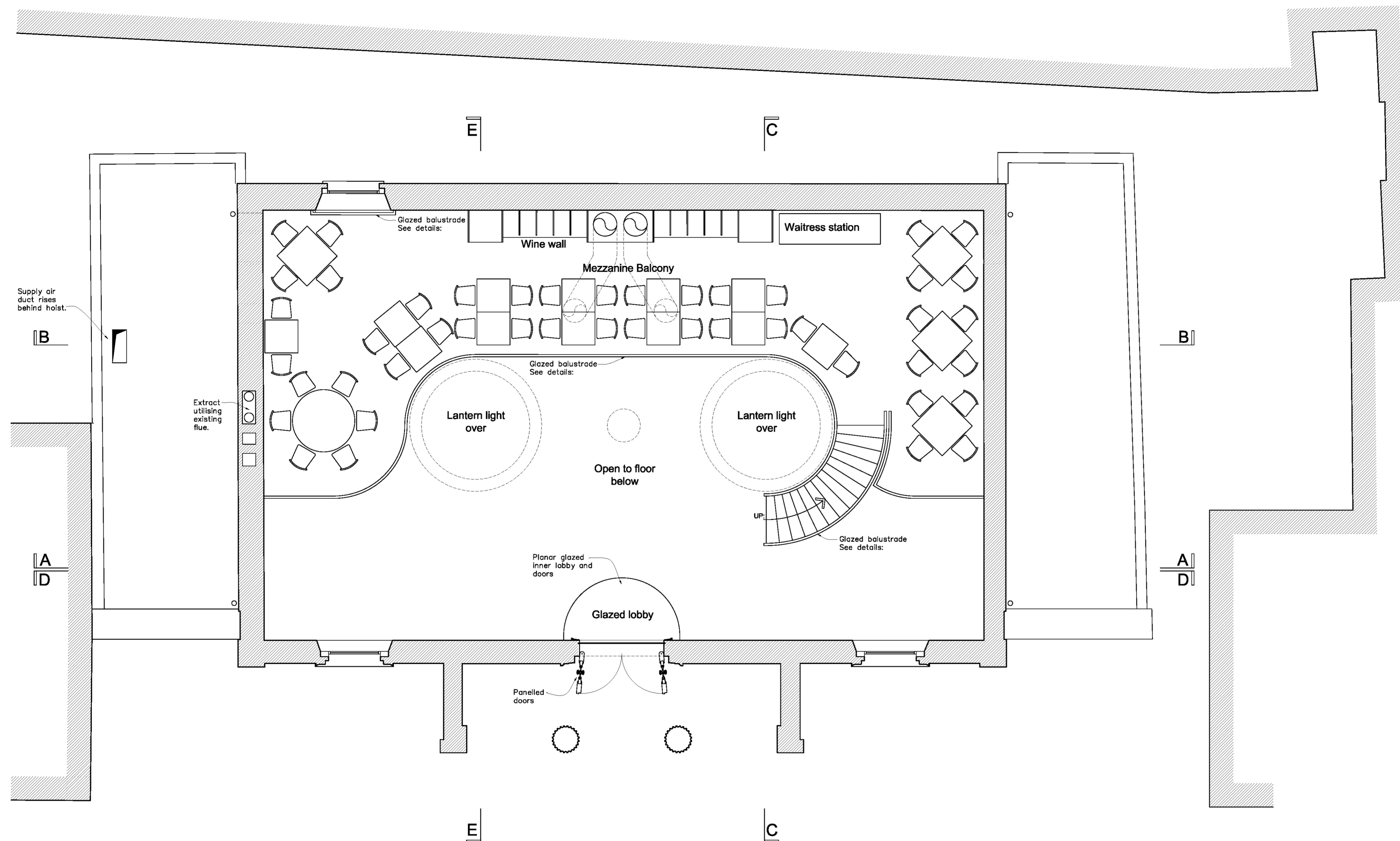
PROPOSED MEZZANINE PLAN
