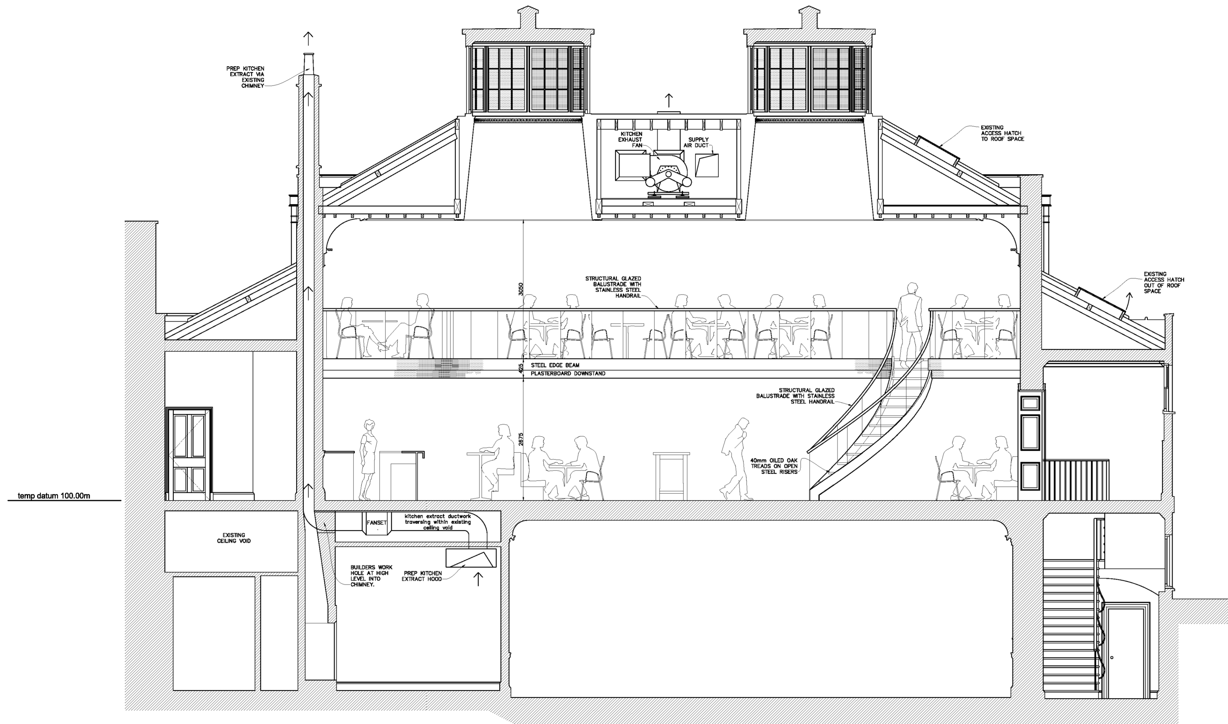
SECTION AA
