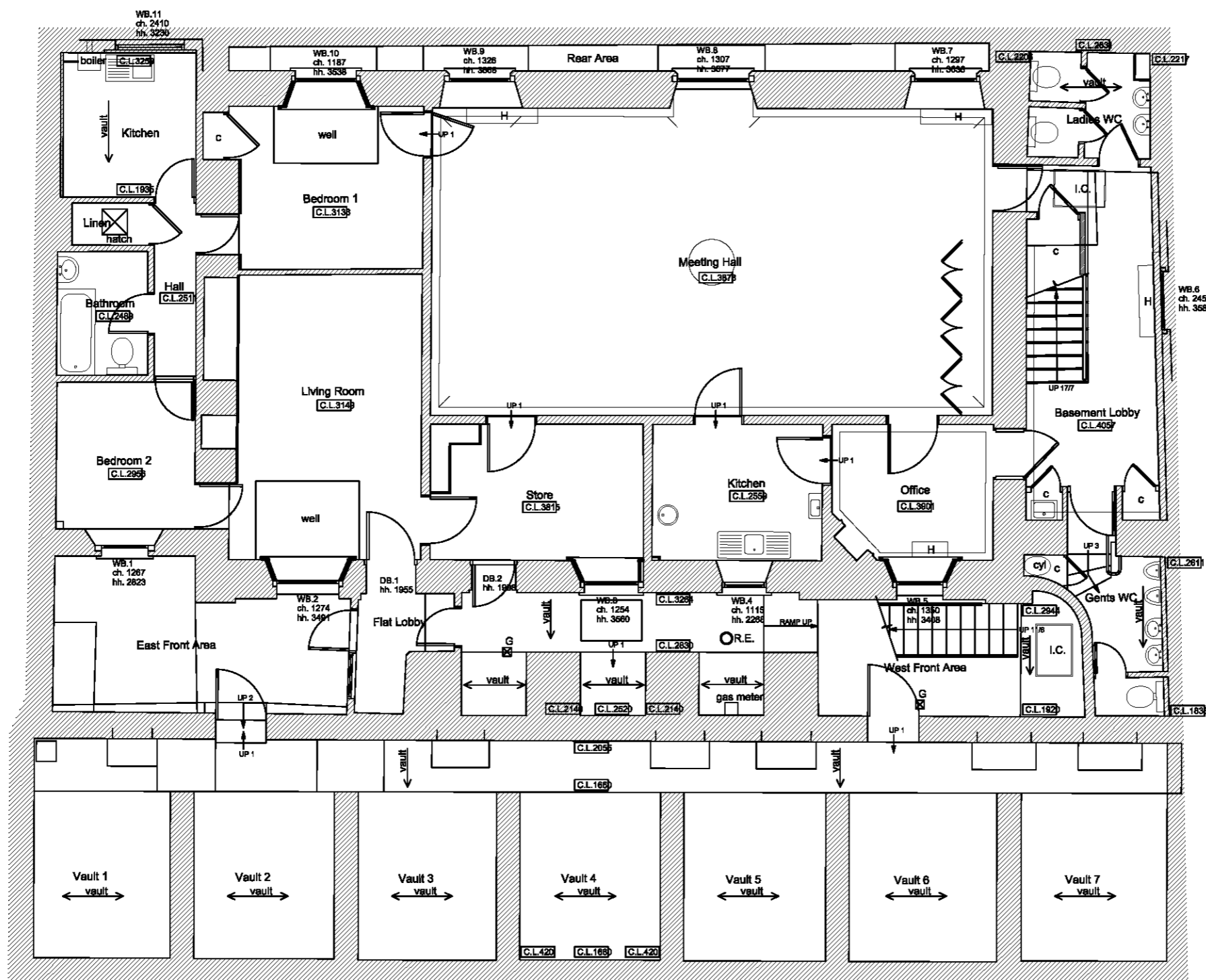
BASEMENT PLAN AS EXISTING
