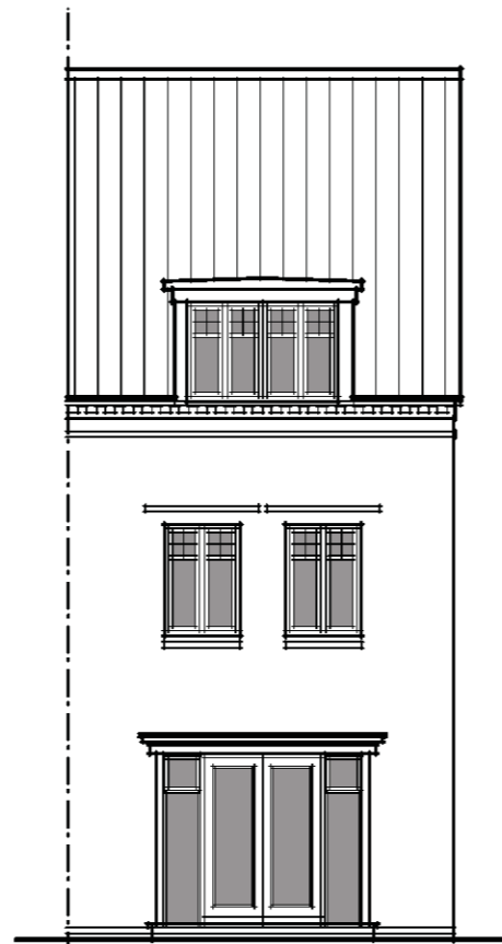
Rear Elevation
