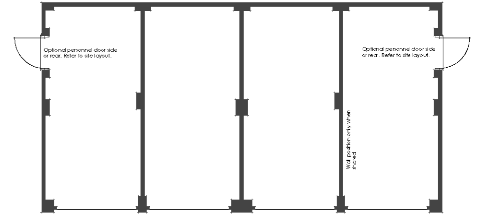
Ground Floor Plan (General)
