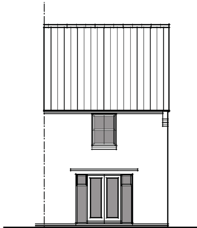
Rear Elevation
