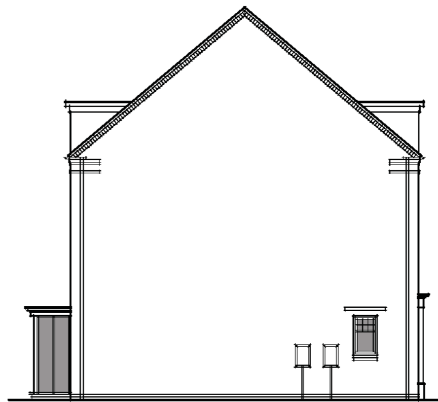
Side Elevation
